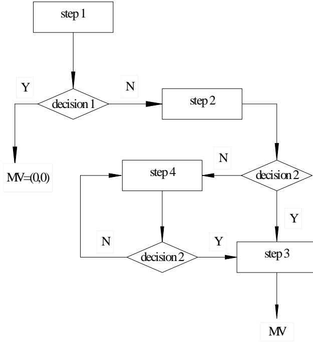
Figure 2: DHCDDS Algorithm's Flow Chart
