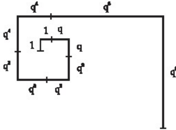
Figure 3: The First Construction Steps of a Polygonal Geometric Spiral with q > 1
