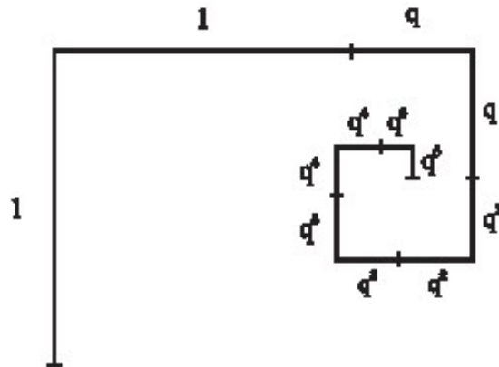
Figure 2: The First Construction Steps of a Polygonal Geometric Spiral with q < 1
